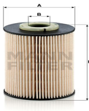
Fuel Filter PU 9003 z EM-20113
